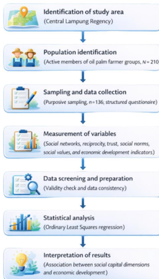
Figure 1. Research Procedure
