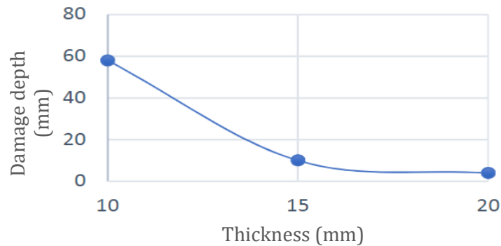
Figure 2. Graph of Test Results Source ( Rahmatullah, Rollastin, & Juanda, 2021 )
