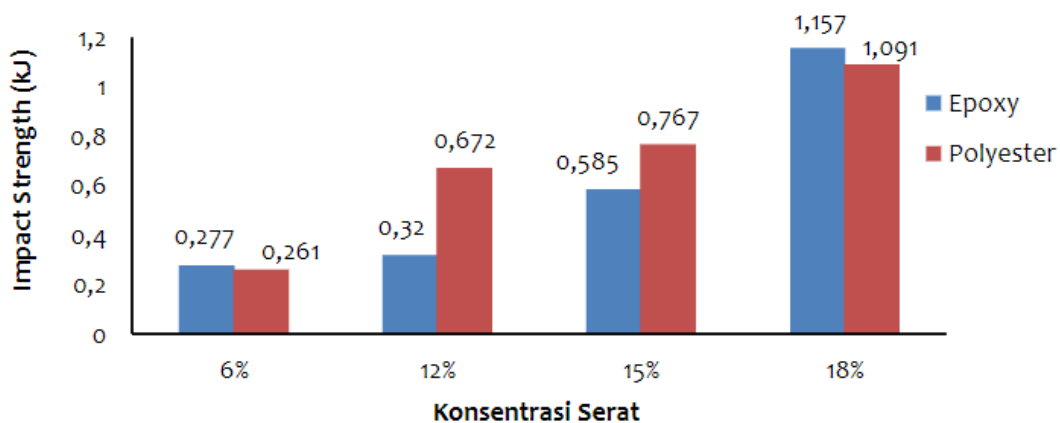
Figure 1. Impact strength of biocomposites
